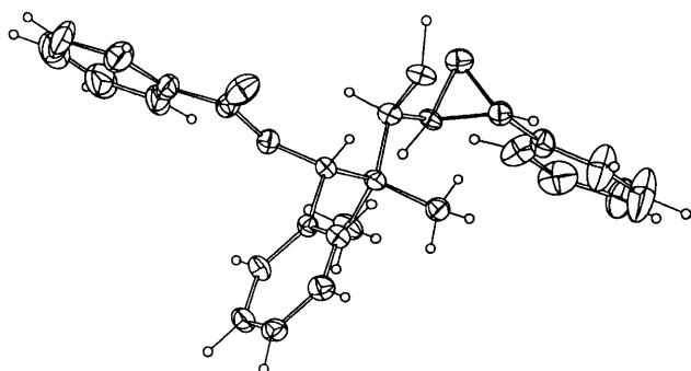
Fig. 1 ORTEP drawing of compound 5a
